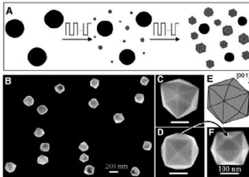
Fig. 6. (a) Scheme of preparation of THH Pt NPs from nanospheres by electrochemical square-wave method. (b) Low-magnification and (c, d, f) high-magnification SEM images of THH Pt NPs. (e) Geometrical model of an ideal THH. Reproduced with permission from Ref. 12 . Copyright ©2007 AAAS.
