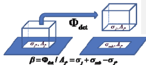
Figure 2. Schematic representation of the detachment of a crystal from a substrate, which changes the contact interface (left) into two new interfaces (right). Reproduced from Ref. 23
